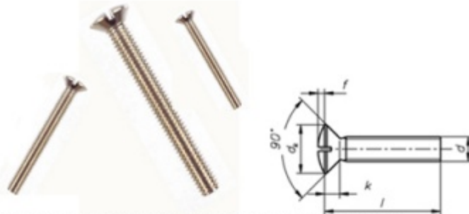
DIN 964 Brass Raised CSK head Screws Brass Slotted DIn 964 Oval head Machine Screws
