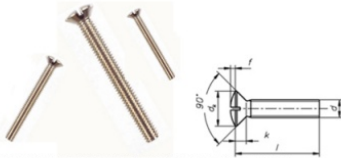
DIN 964 Brass Raised CSK head Screws Brass Slotted DIn 964 Oval head Machine Screws
